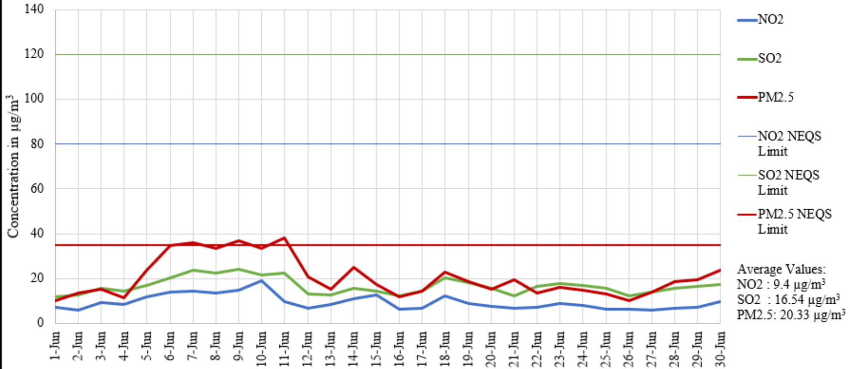
Graphical Representation of Concentrations of PM 2.5 , NO 2 , and SO 2 in Islamabad for June 2021
