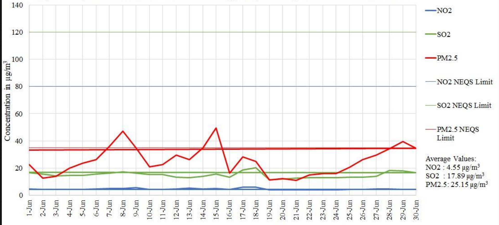
Graphical Representation of Concentrations of PM 2.5 , NO 2 , and SO 2 in Islamabad for June, 2022
