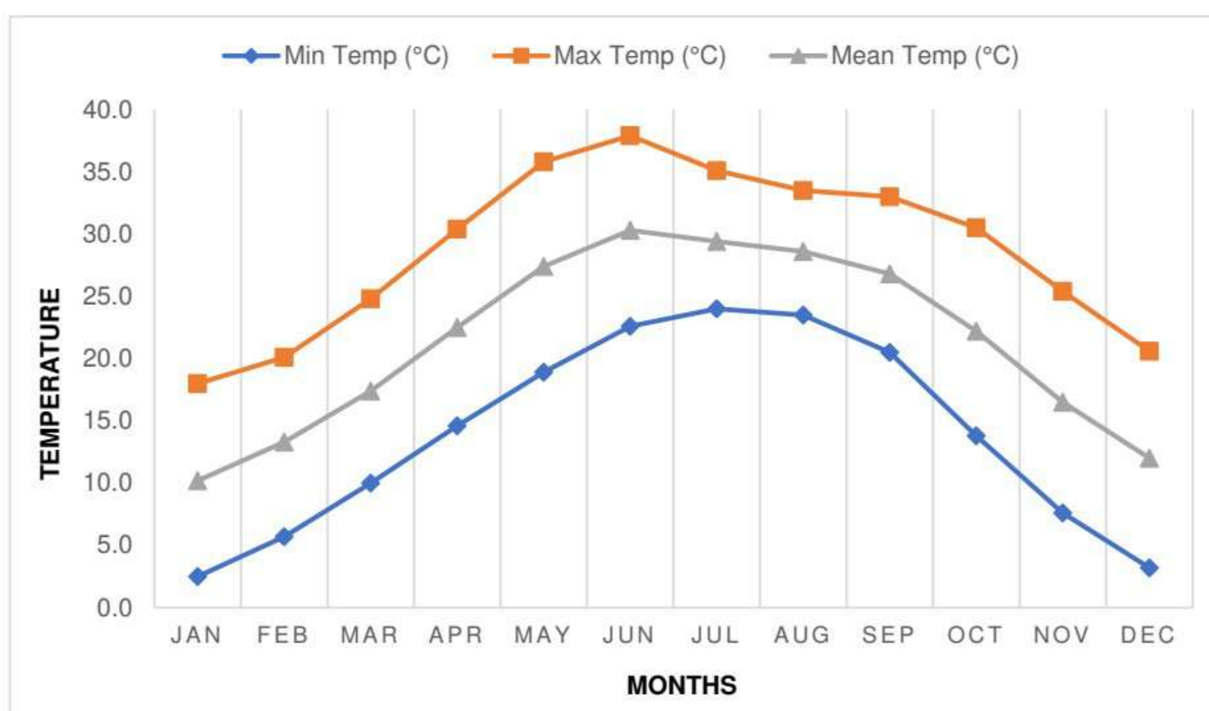
Figure 2.5: Mean Monthly Temperatures in Islamabad
