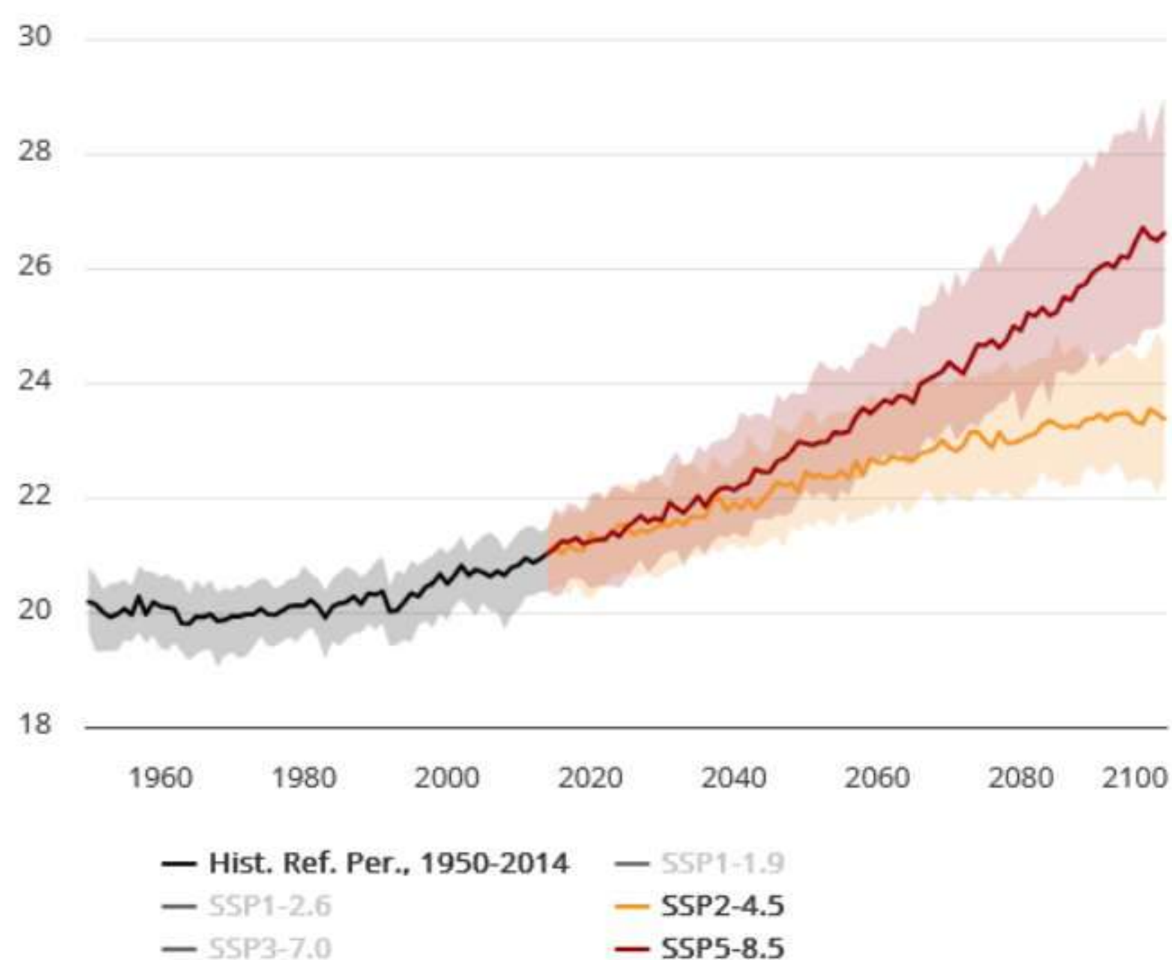
Figure 1.5: Projected Mean Temperature (Multi-Model Ensemble) Pakistan
