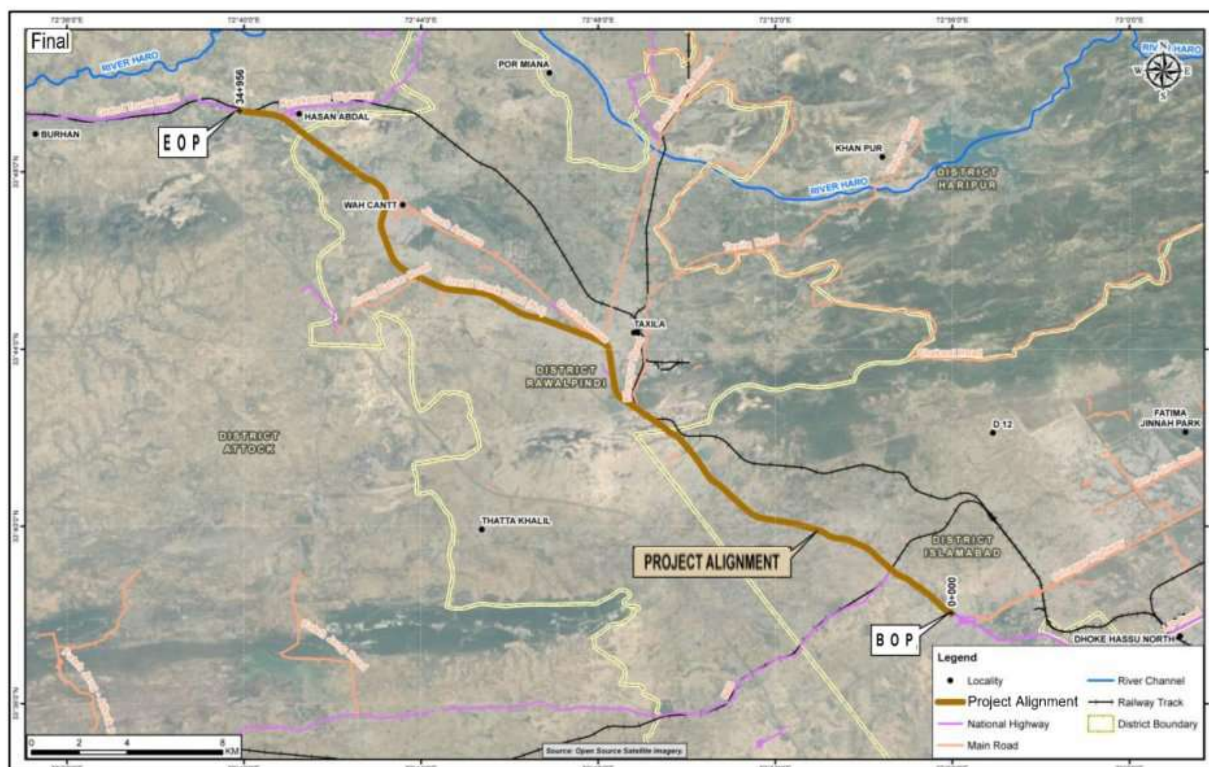
Figure 2.1: Location Map of Project Area
