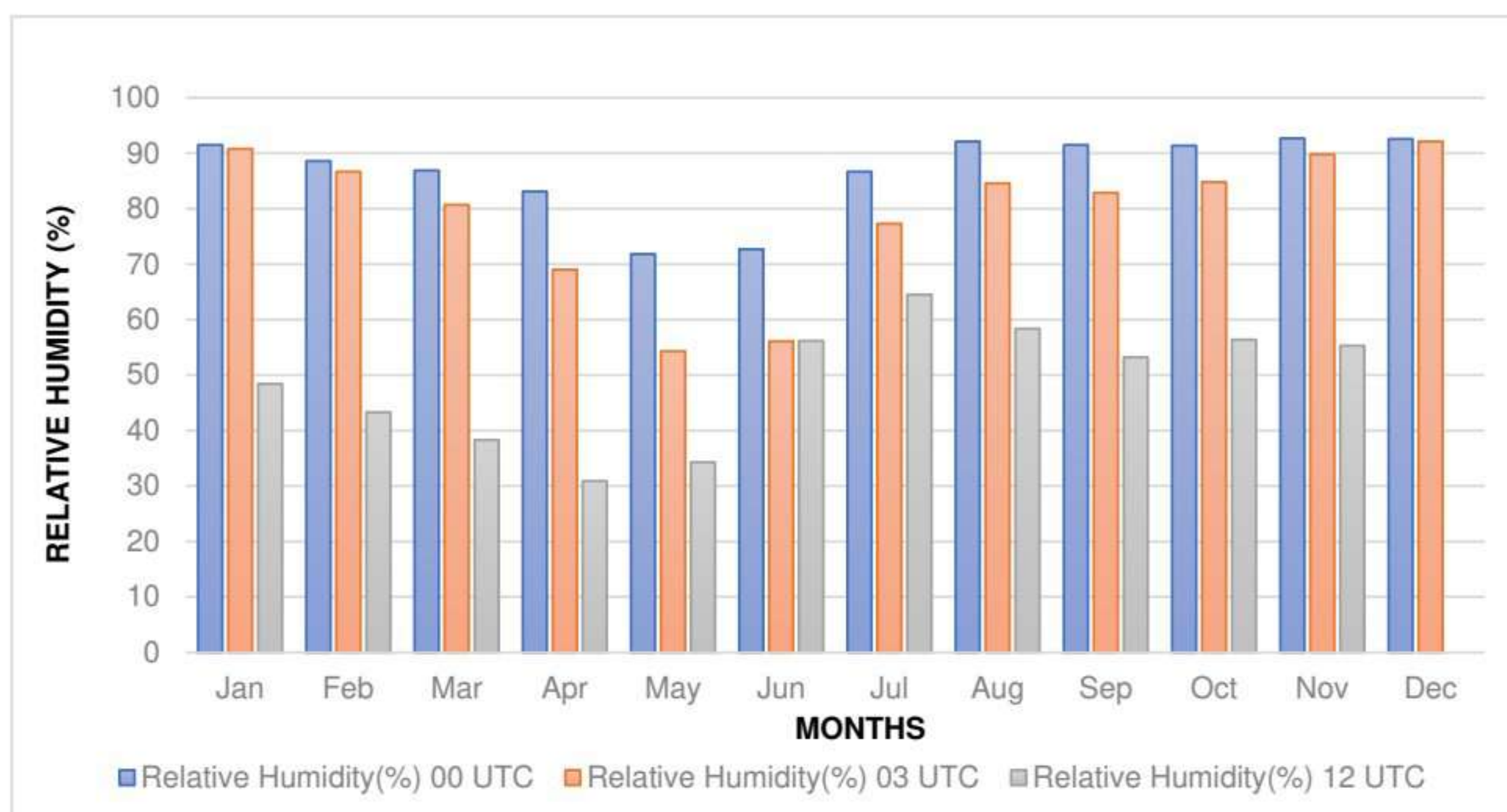
Figure 2.6: Monthly Relative Humidity in Islamabad
