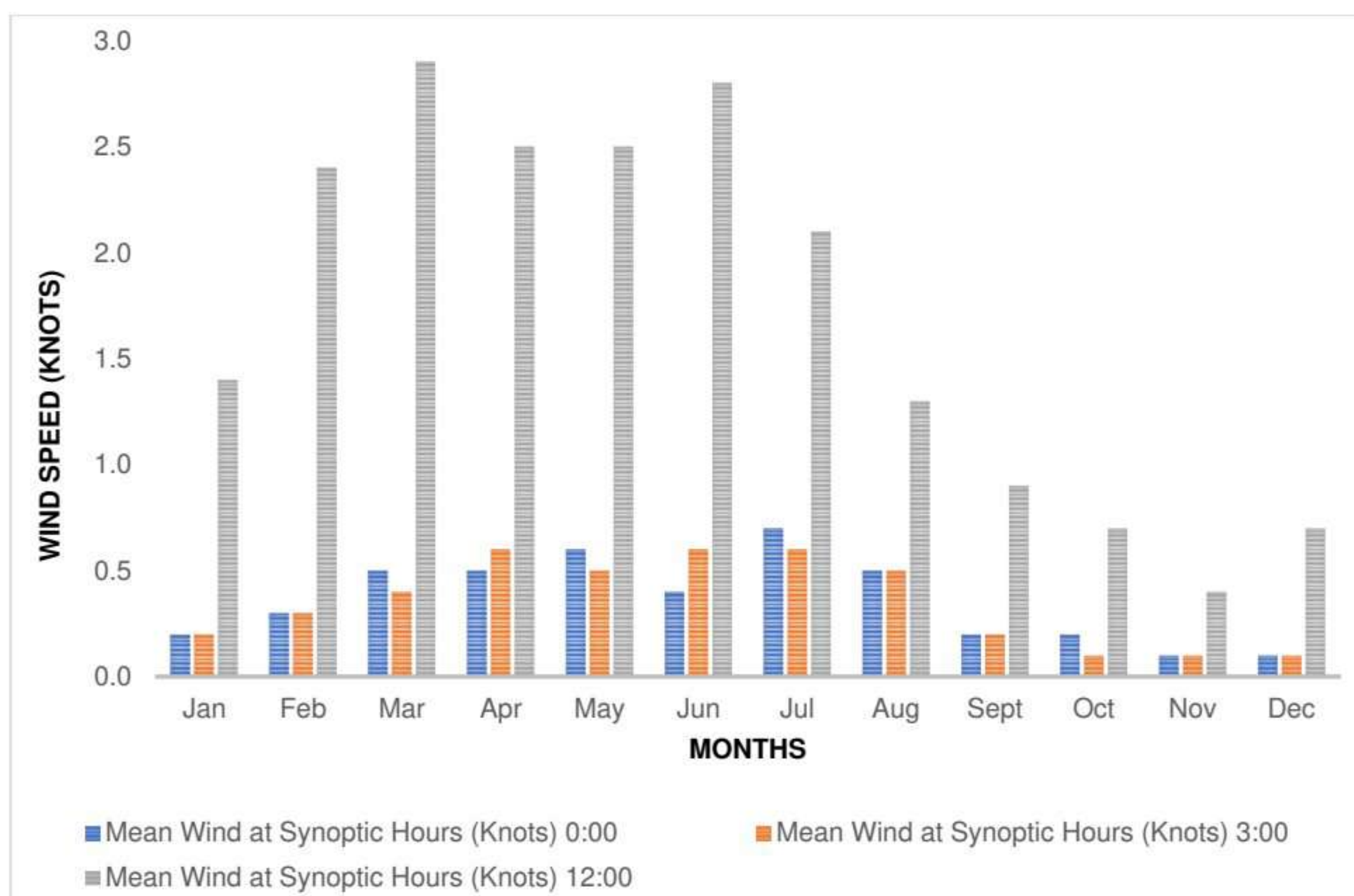
Figure 2.7: Mean Monthly Wind Speed in Islamabad
