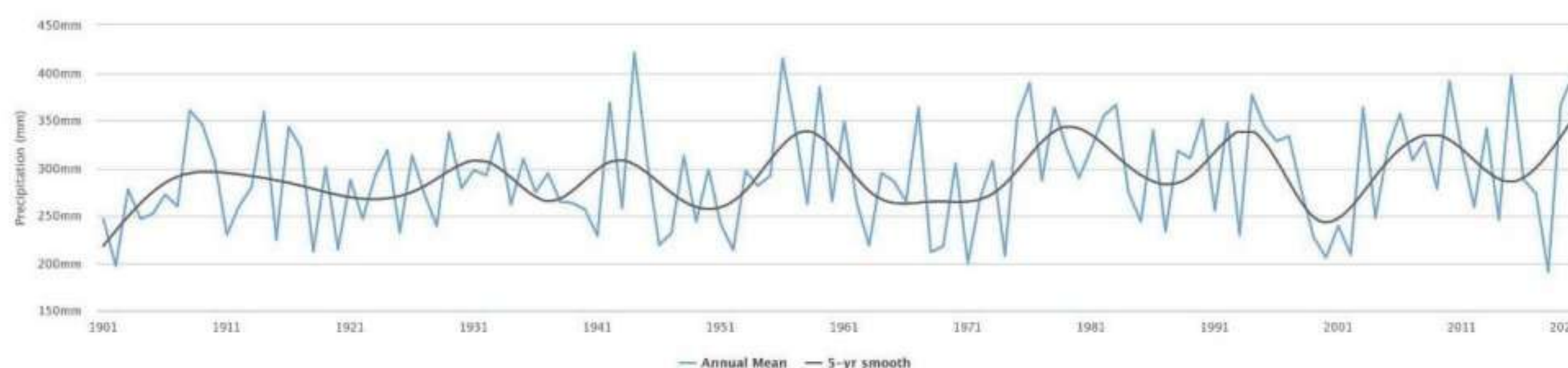
Figure 1.4: Observed Average Annual Rainfall of Pakistan for 1901-2020
