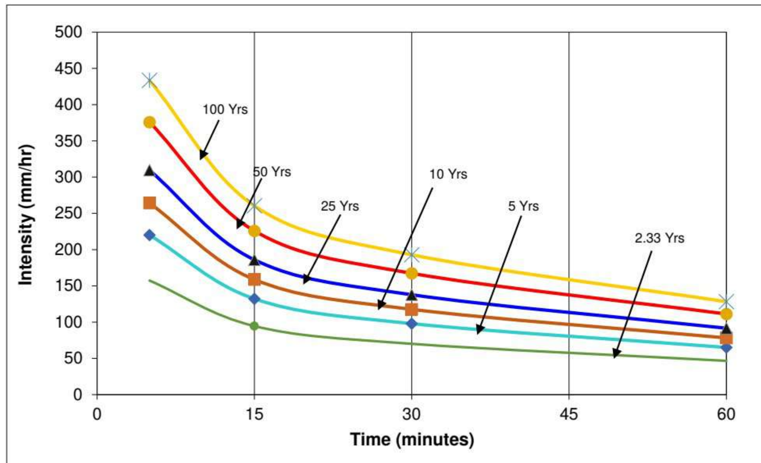
Figure 2.15: Intensity-Duration-Frequency Curve for Islamabad
