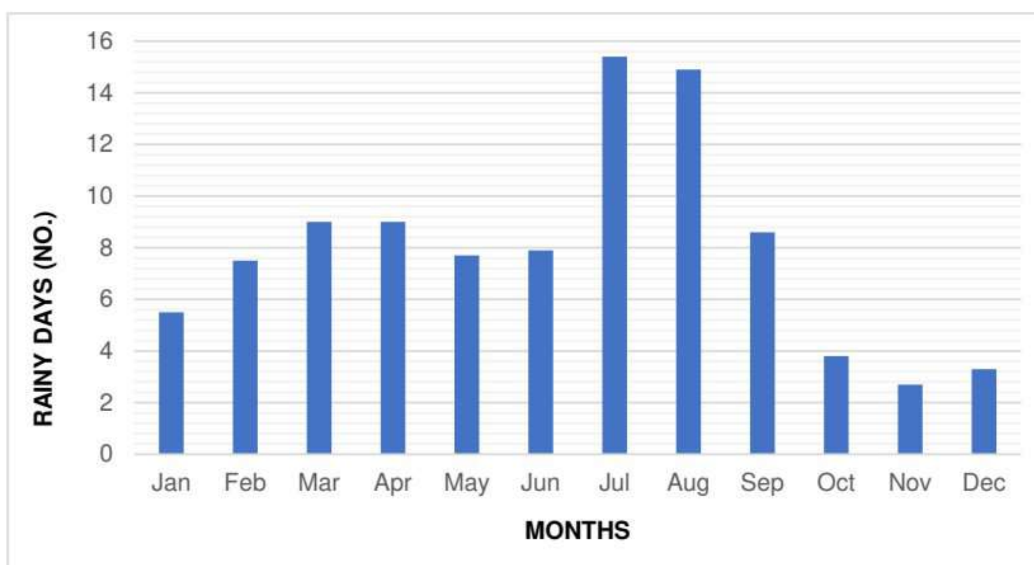
Figure 2.4: Number of Rainy Days in Islamabad
