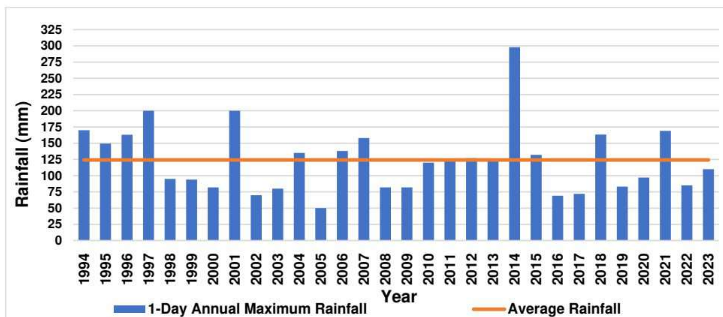
Figure 2.13: One-Day Annual Maximum Rainfall in Islamabad
