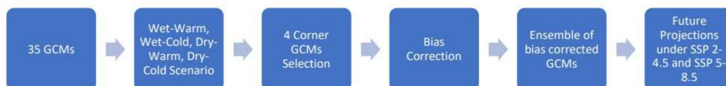
Figure 1.9: Overall Methodology Adopted for Climate Change Study
