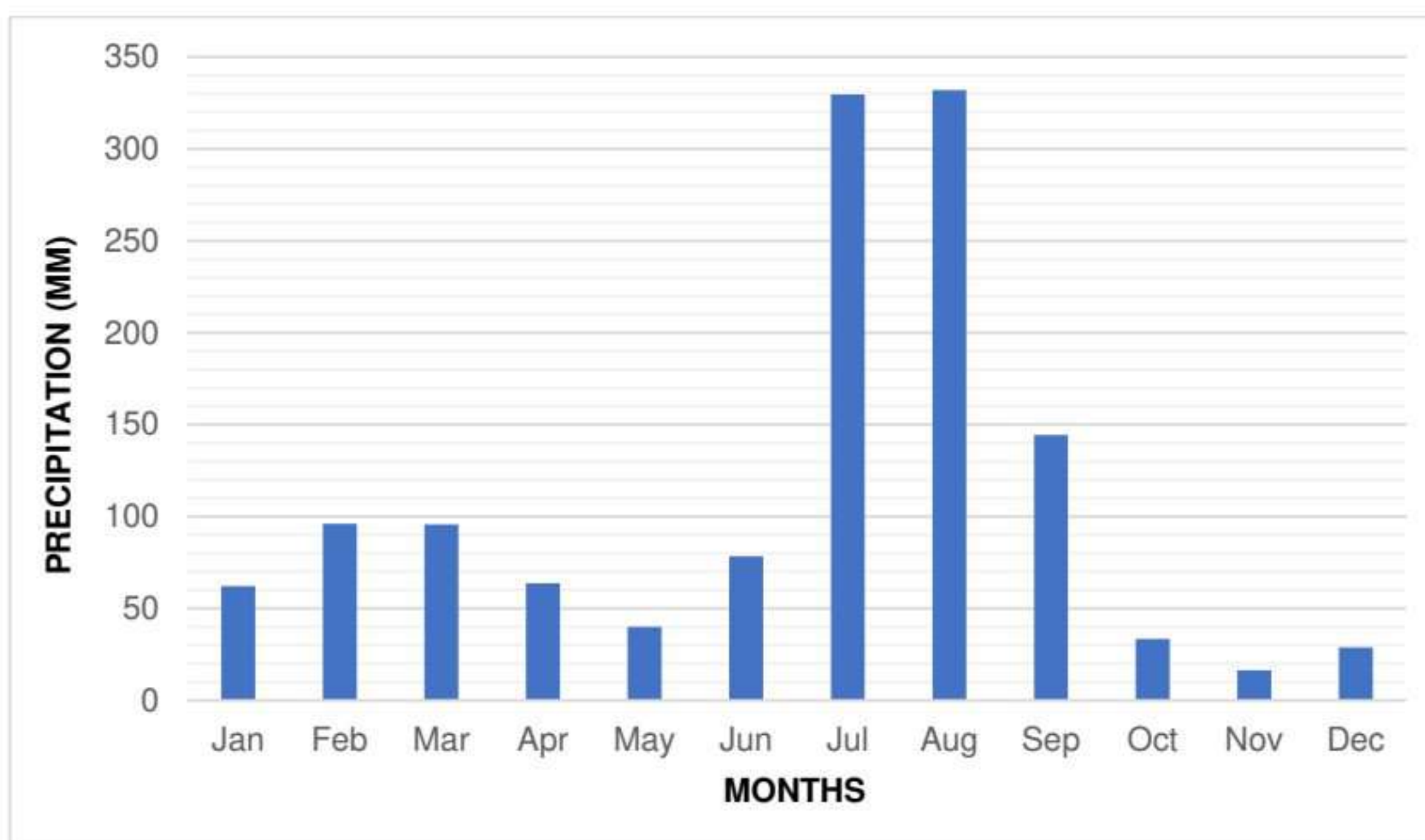
Figure 2.3: Mean Monthly Distribution of Rainfall in Islamabad
